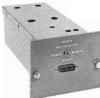
Audio Input Control Module
