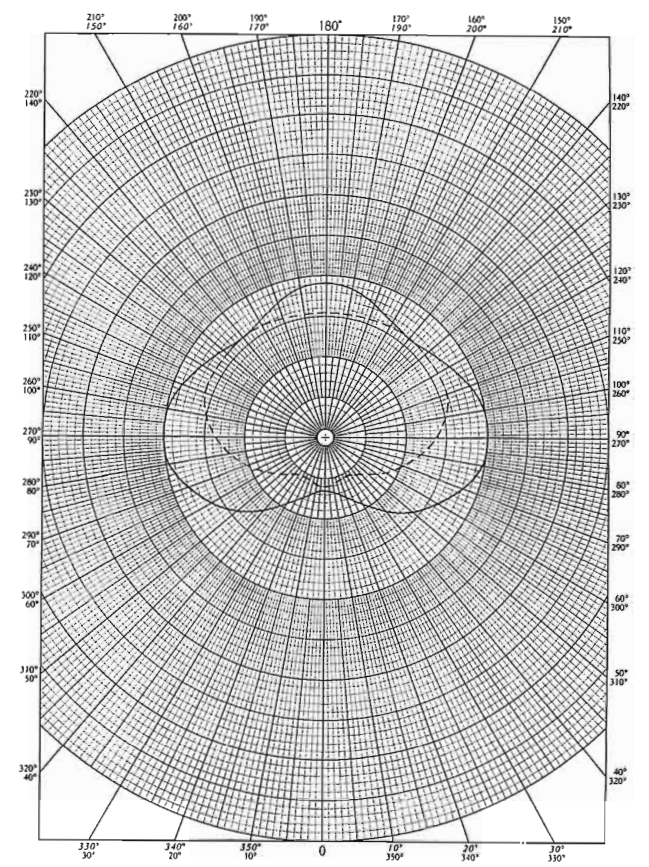
PATTERN "B" Horizontal Relative Field Patterns
