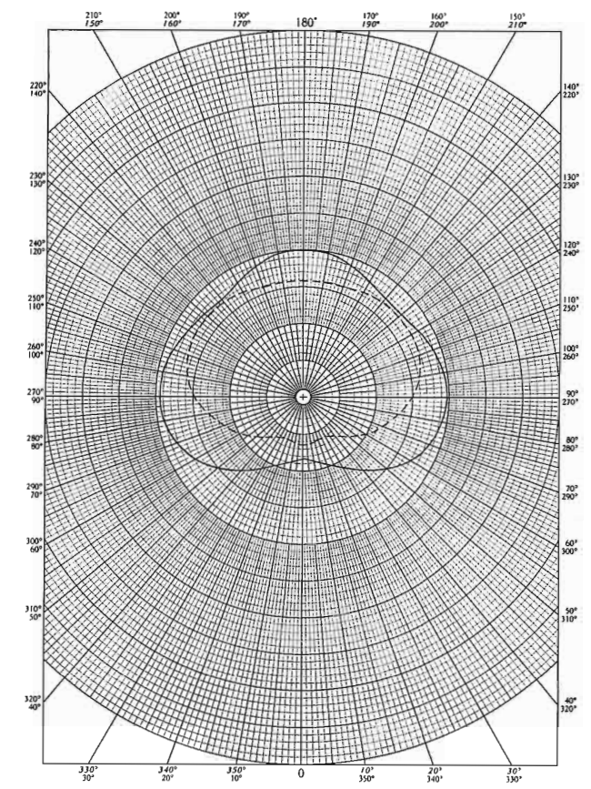
PATTERN "A" Horizontal Relative Field Patterns
