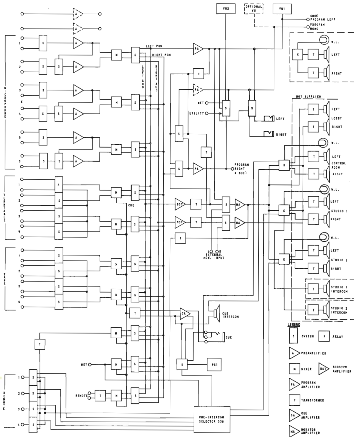
BLOCK DIAGRAM EXECUTIVE
