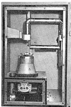
Driver amplifier located directly below the 4CX5000A power amplifier for added efficiency of operation.
